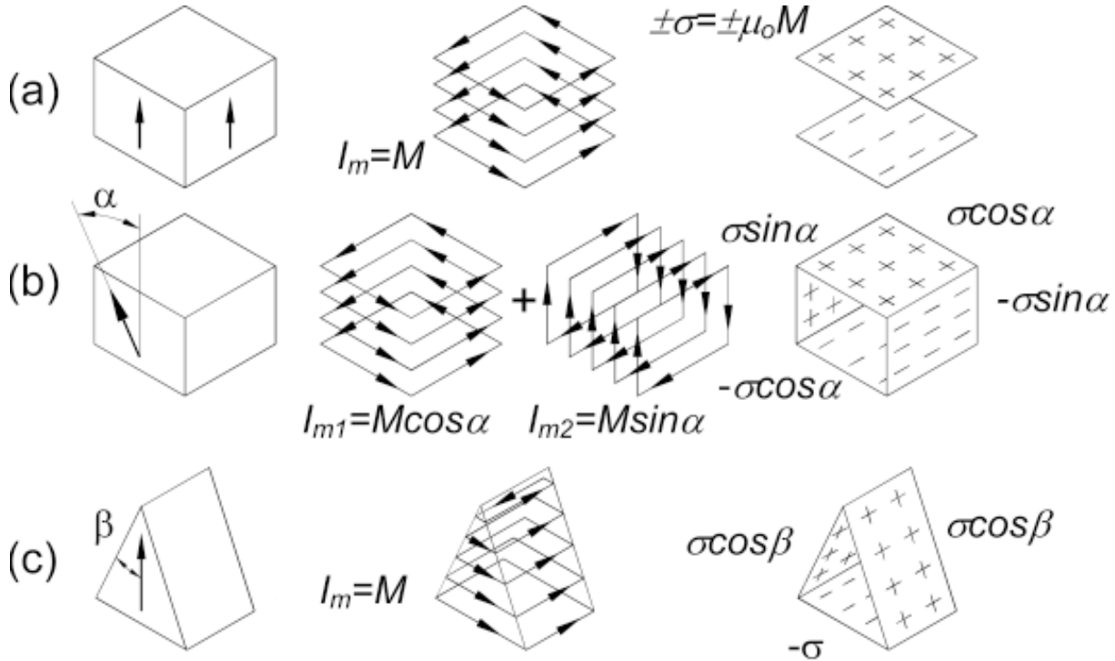
Fig. 1. Presentation of prismatic magnets (left column) by Amperian currents (middle column) and surface magnetic charges (right column).
